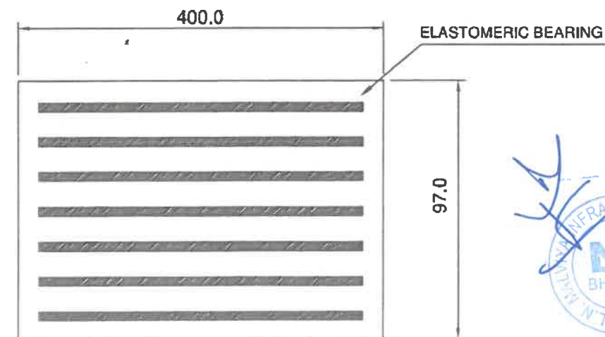
ARRANGEMENT OF BEARING
