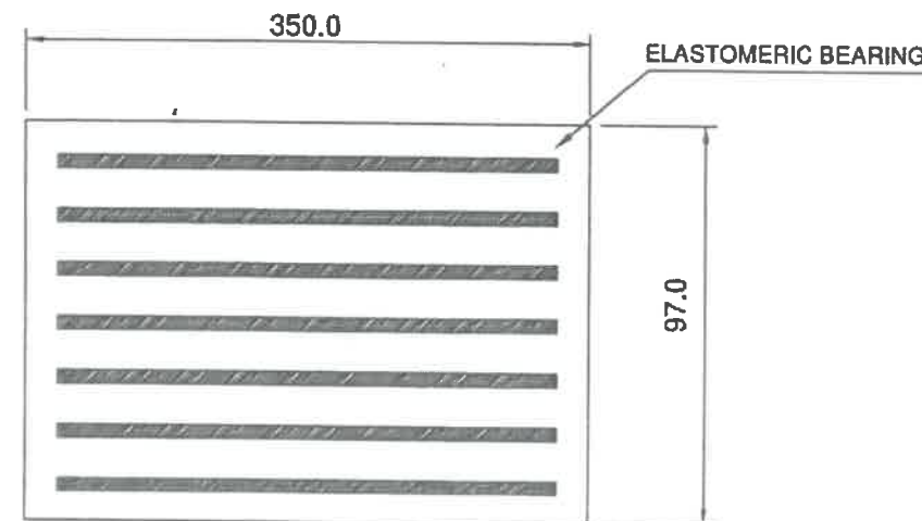
ARRANGEMENT OF BEARING
