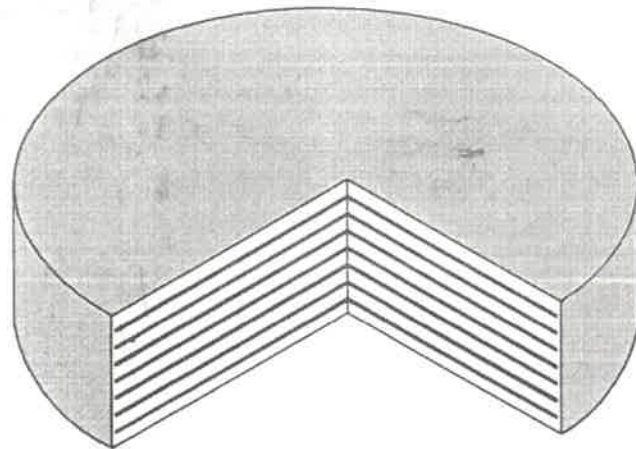
ISOMETRIC VIEW OF CIRCULAR ELASTOMERIC BEARING THE NUMBER OF STEEL LAMINATES AND ELASTOMERS ARE INDICATIVE ONLY. THE NUMBER SHALL NOT BE COUNTED, ONLY THE PROVIDED INFORMATION IN THE SECTION X - X SHALL BE REFERRED
