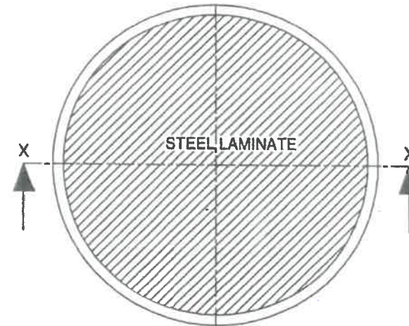
PLAN OF ELASTOMERIC BEARING ( PLAN SHOWING STEEL LAMINATE )
