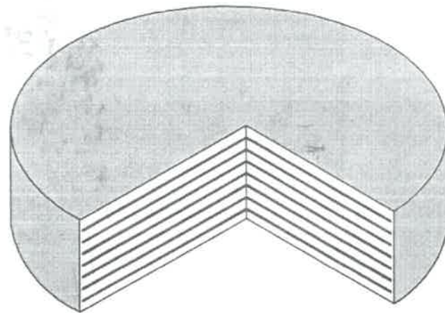
ISOMETRIC VIEW OF CIRCULAR ELASTOMERIC BEARING
