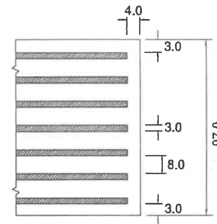
DETAILS 'A'
