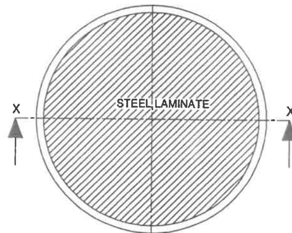
PLAN OF ELASTOMERIC BEARING ( PLAN SHOWING STEEL LAMINATE )
